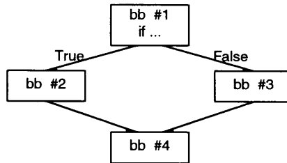
Figure 5-2. Flow Graph
